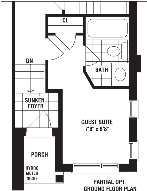
PARTIAL OPT. GROUND FLOOR PLAN ELEV. 'B' (UPGRADE) W/GUEST SUITE
