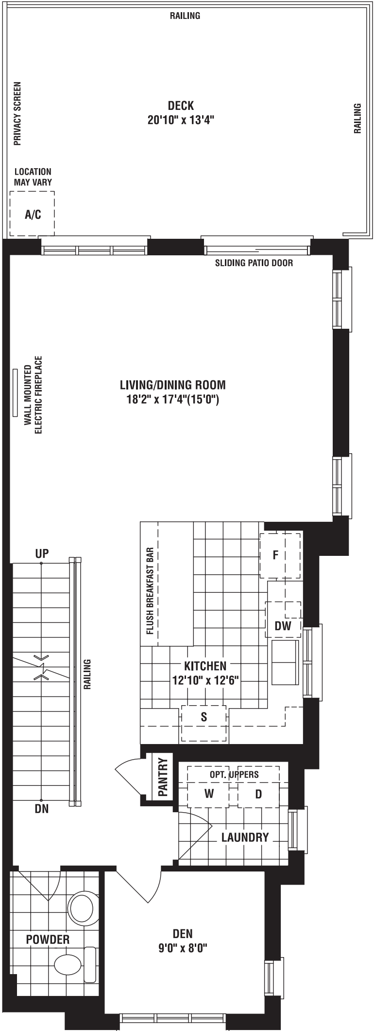
MAIN FLOOR PLAN ELEV. 'A'
