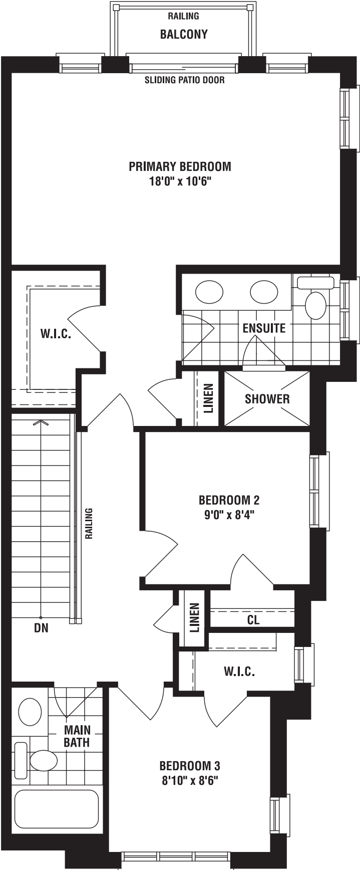
UPPER FLOOR PLAN ELEV. 'A'
