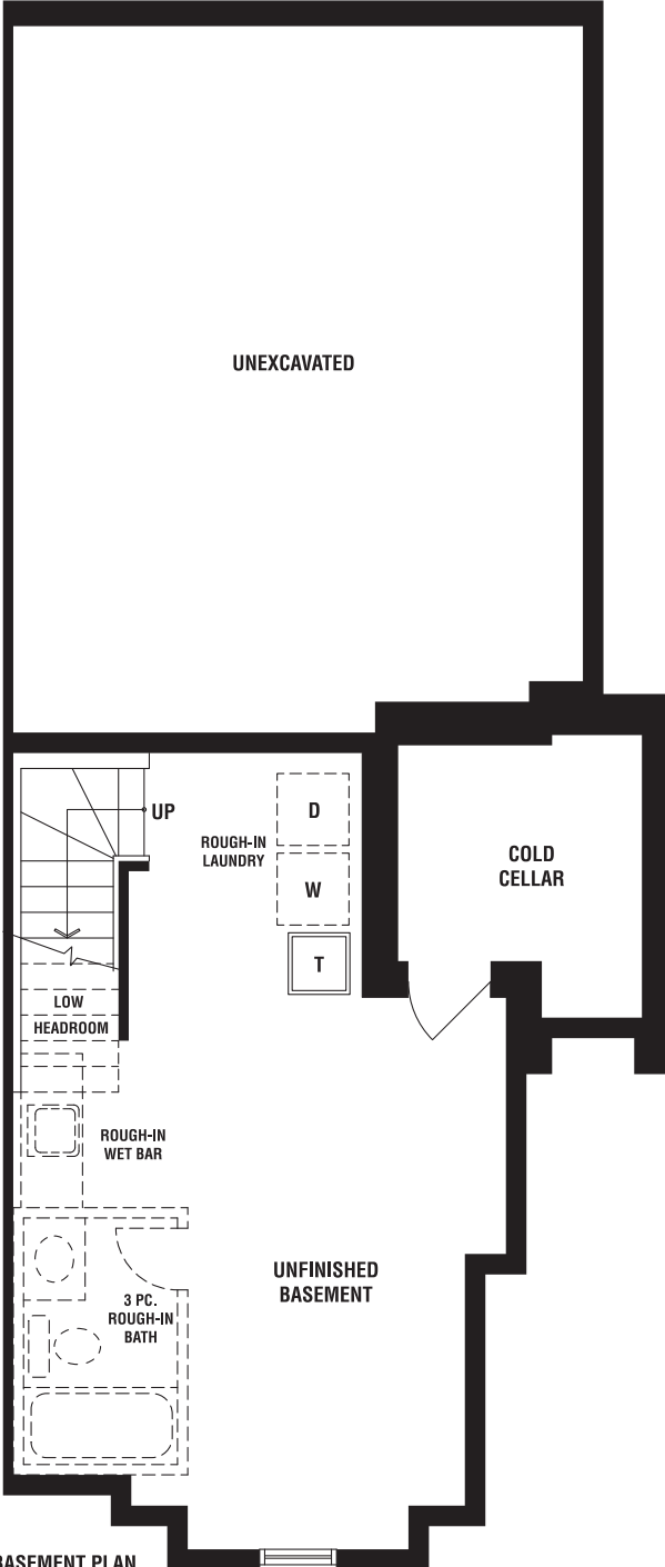
BASEMENT PLAN ELEV. 'A'
