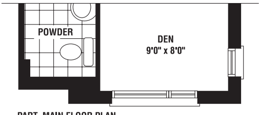
PART. MAIN FLOOR PLAN ELEV. 'B'
