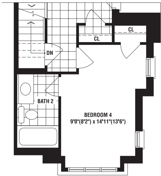
PART. OPT. GROUND FLOOR PLAN ELEV. 'A' W/ BEDROOM 4
