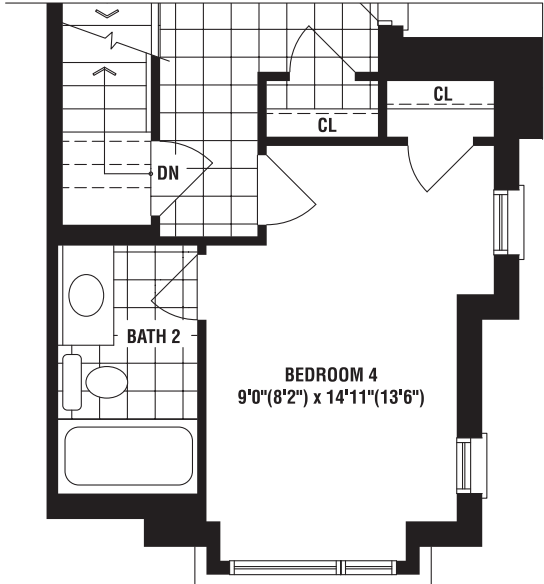
PART. OPT. GROUND FLOOR PLAN ELEV. 'B' W/ BEDROOM 4
