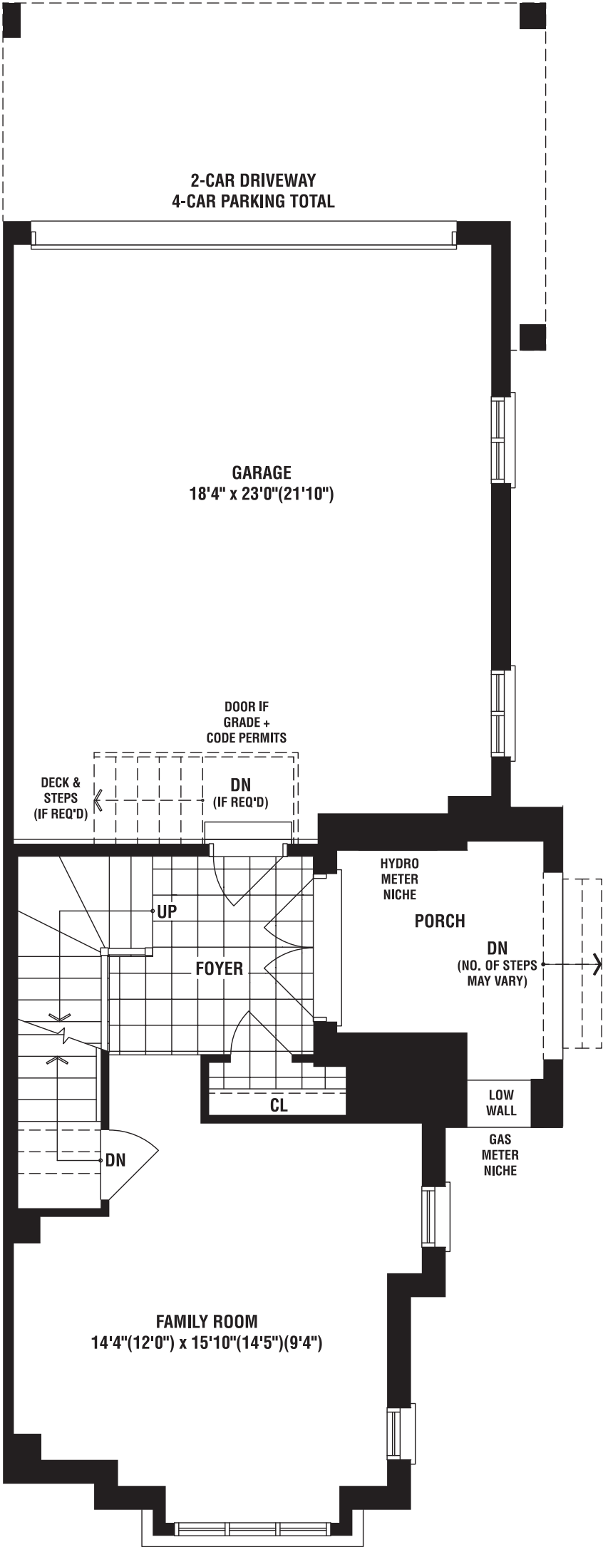
GROUND FLOOR PLAN ELEV. 'A'
