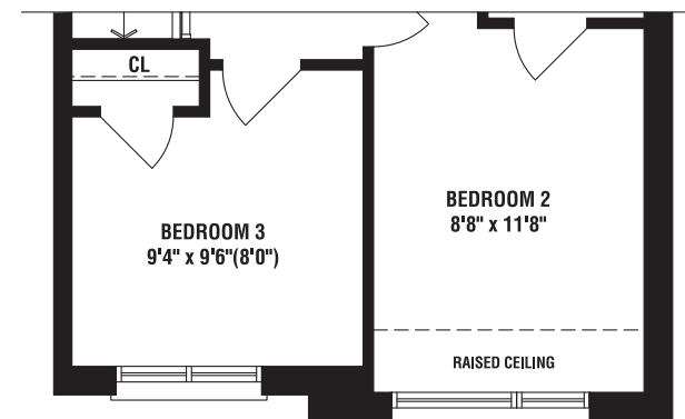
PARTIAL UPPER FLOOR PLAN 3 BEDROOM & 2 BATH ELEV. 'B'
