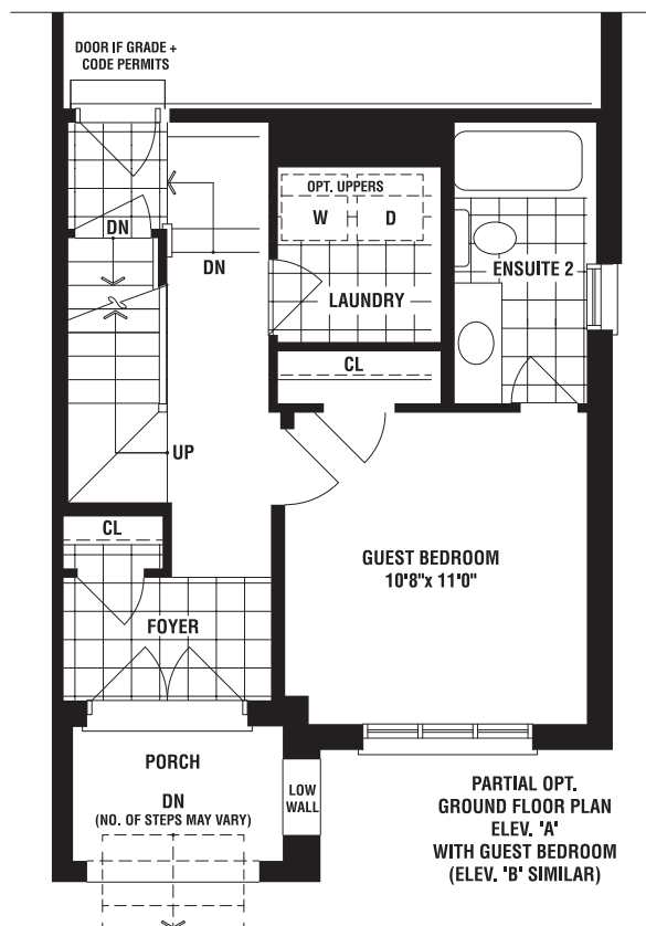
GROUND FLOOR PLAN ELEV. 'A'
