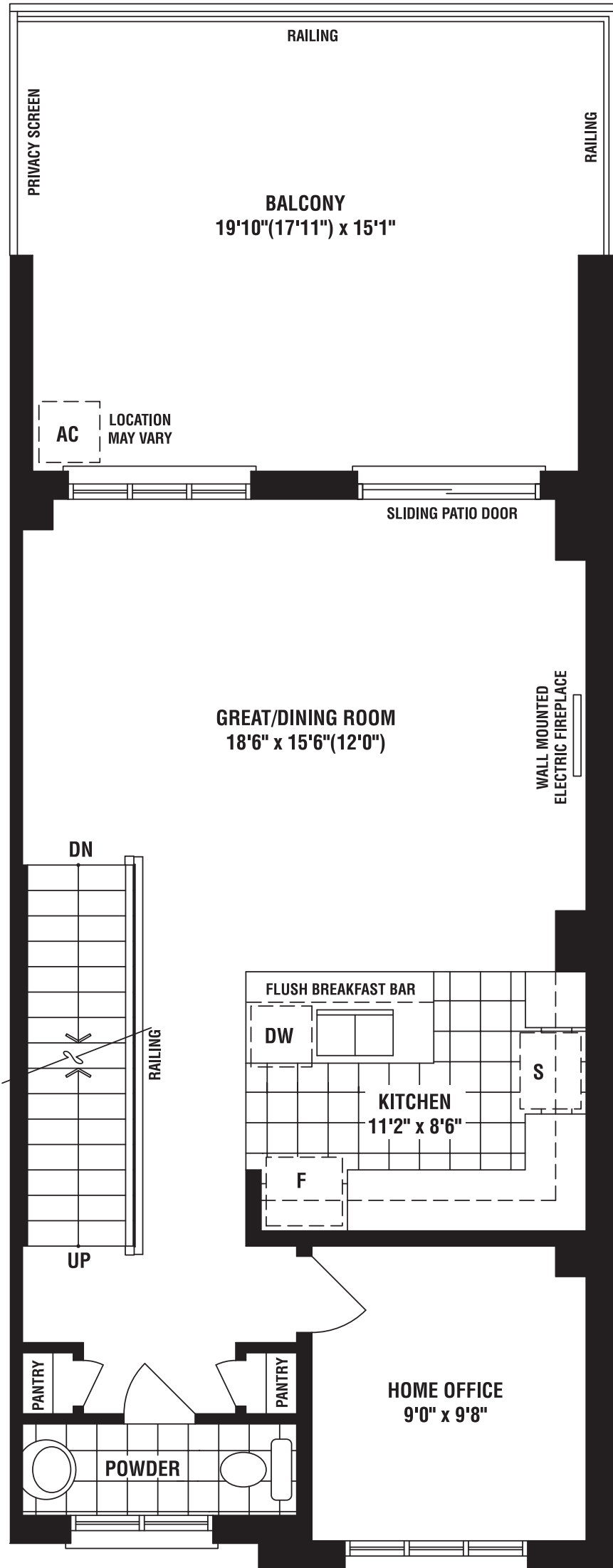
MAIN FLOOR PLAN ELEV. 'A'
