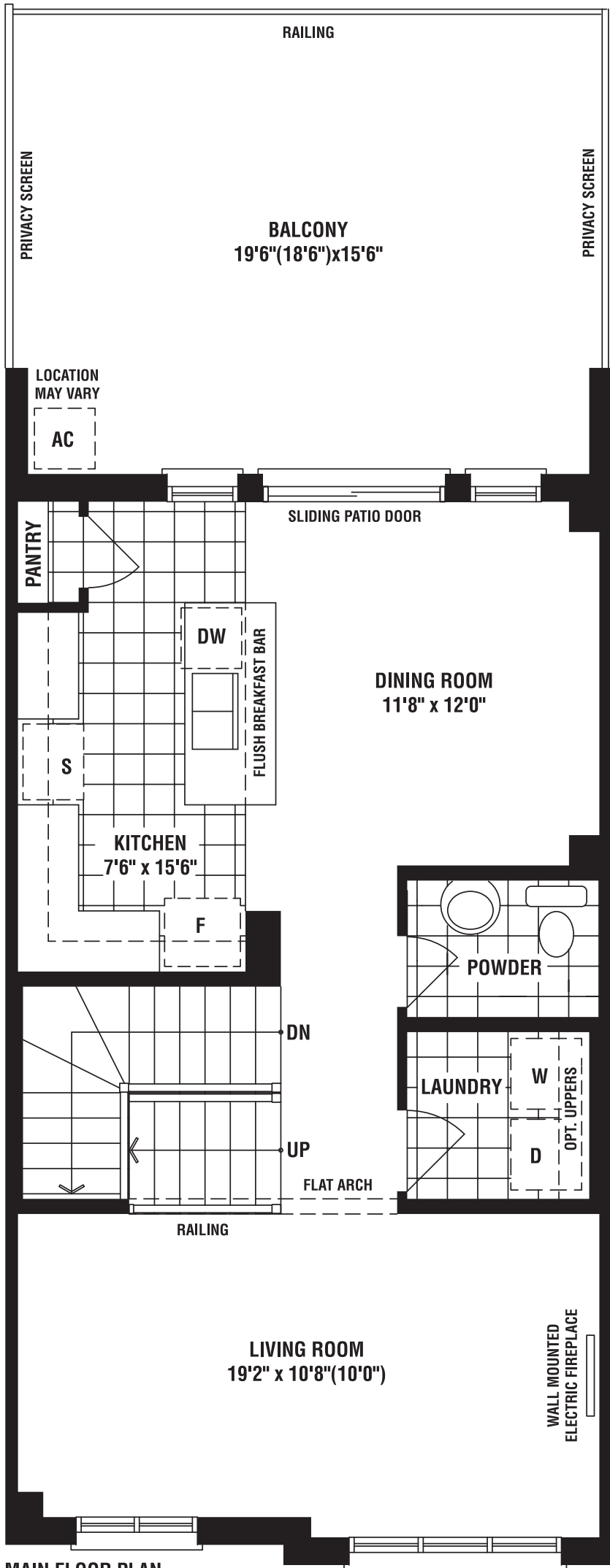
MAIN FLOOR PLAN ELEV. 'A'
