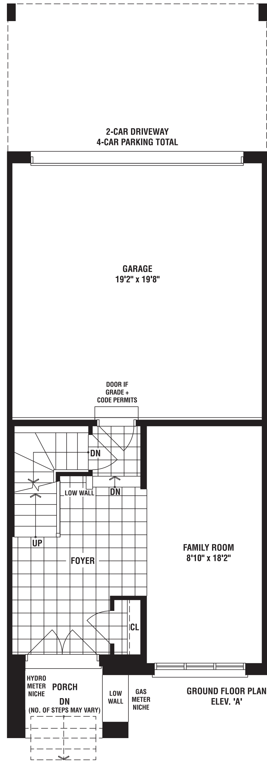
MAIN FLOOR PLAN ELEV. 'A'
