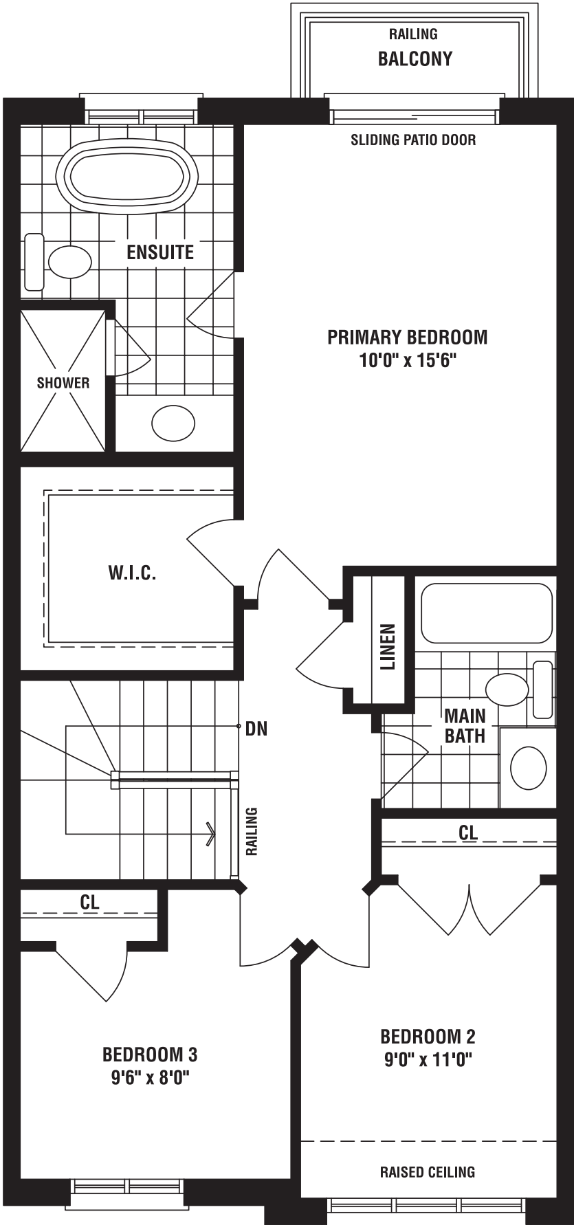
UPPER FLOOR PLAN 3 BEDROOM & 2 BATH ELEV. 'A'
