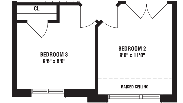
PARTIAL UPPER FLOOR PLAN 3 BEDROOM & 2 BATH ELEV. 'B'
