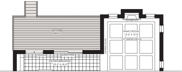
PARTIAL GROUND FLOOR ELEV. 'B' LOOK OUT BASEMENT CONDITION
