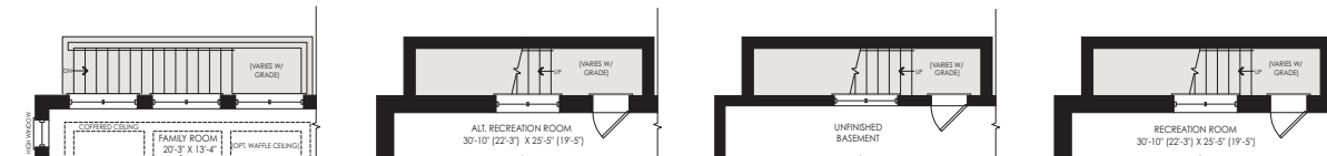
PARTIAL GROUND FLOOR FOR WALK-UP BASEMENT
