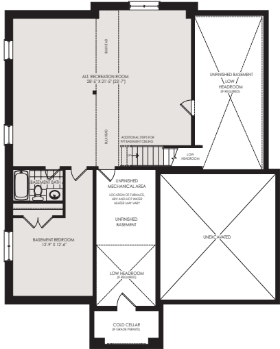
OPT. FINISHED BASEMENT PLAN W/ BASEMENT BEDROOM & BATHROOM ELEV. 'A' (STANDARD BASEMENT CEILING HEIGHT)
