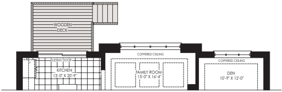
PARTIAL GROUND FLOOR ELEV. 'B' LOOK OUT BASEMENT CONDITION
