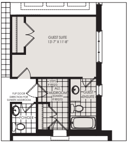
PARTIAL GROUND FLOOR OPT. GUEST SUITE ELEV. 'B'
