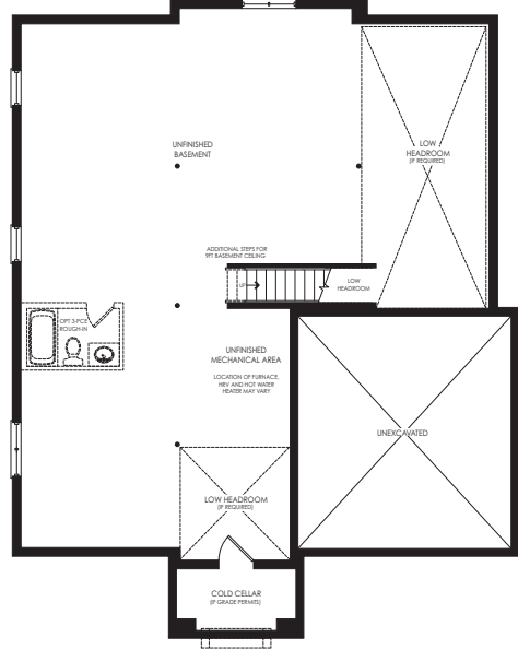
BASEMENT PLAN ELEV. 'A'
