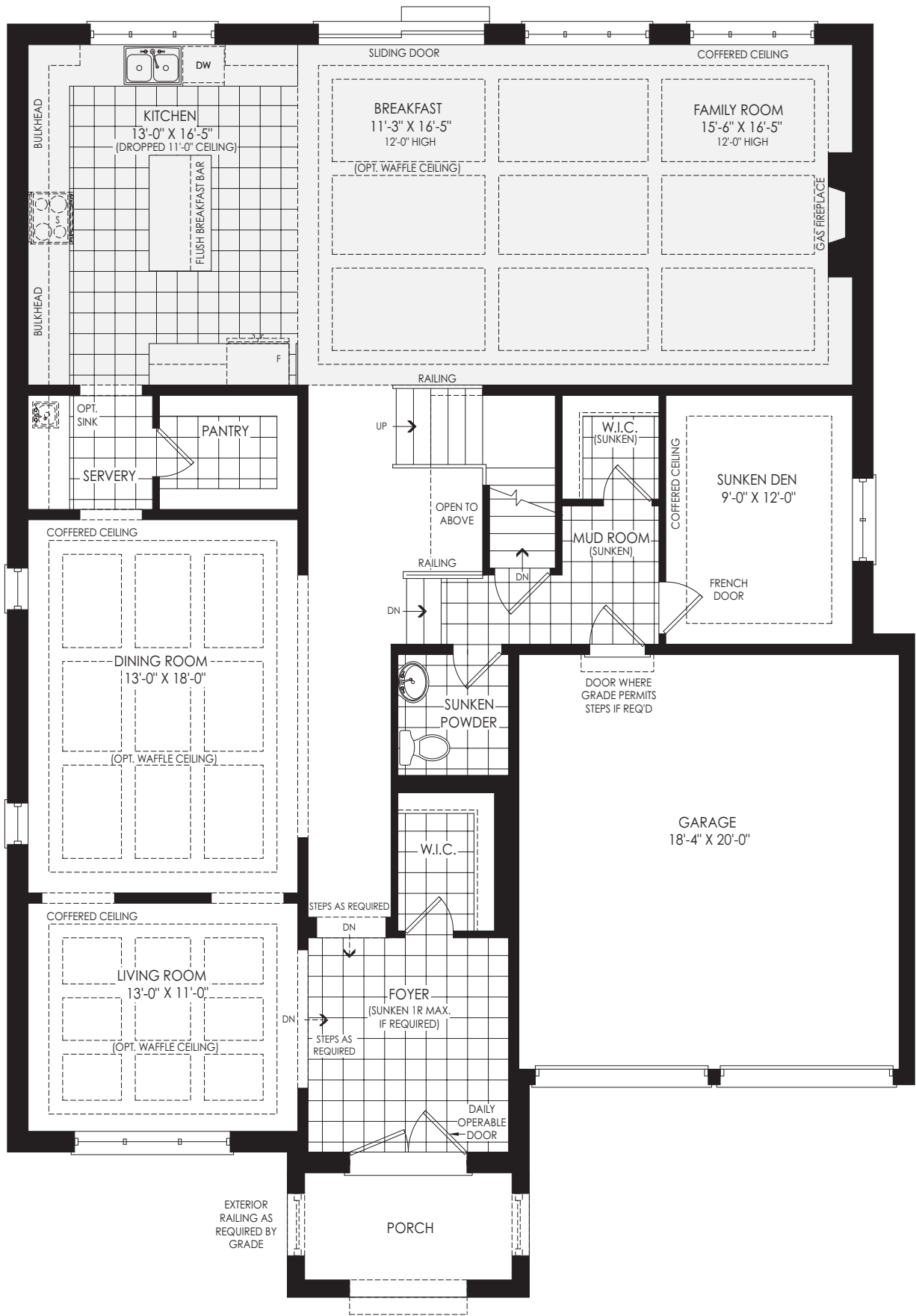
GROUND FLOOR PLAN ELEV. 'C'
