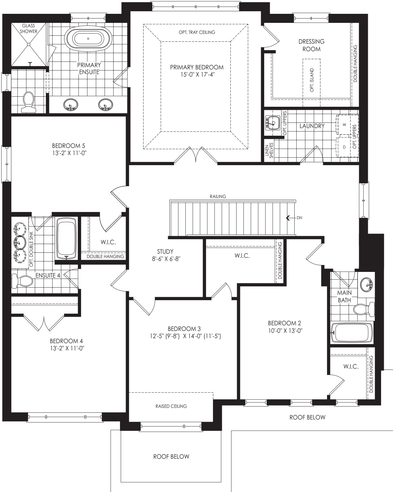
SECOND FLOOR PLAN ELEV. 'A'
