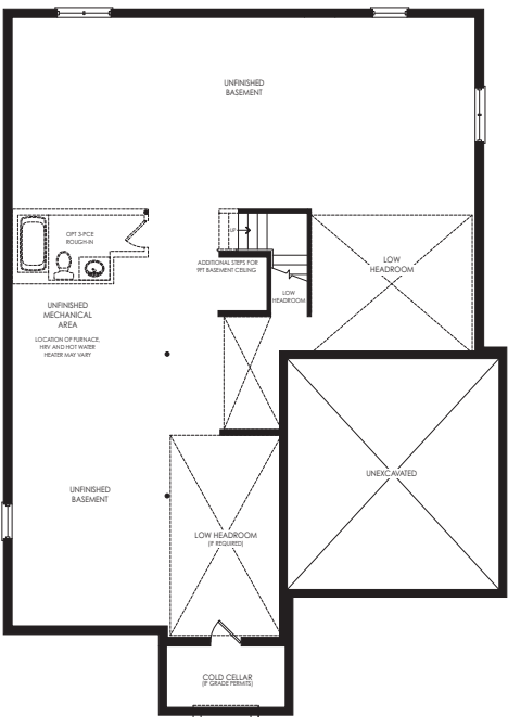
BASEMENT PLAN ELEV. 'C'
