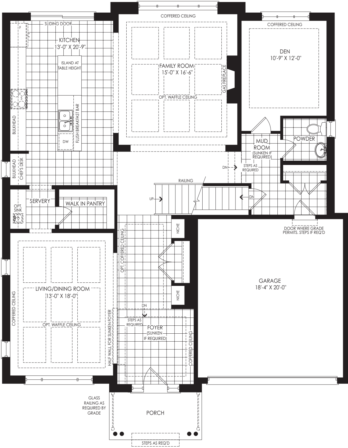
GROUND FLOOR PLAN ELEV. 'A'
