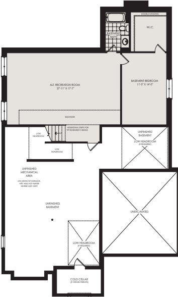
OPT. FINISHED BASEMENT PLAN W/ 3 PC. BATHROOM & BATHROOM ELEV. 'B' (STANDARD BASEMENT CEILING HEIGHT)
