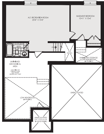
OPTIONAL FINISHED BASEMENT WITH RECREATION ROOM, BEDROOM AND BATHROOM ELEV. 'A'
