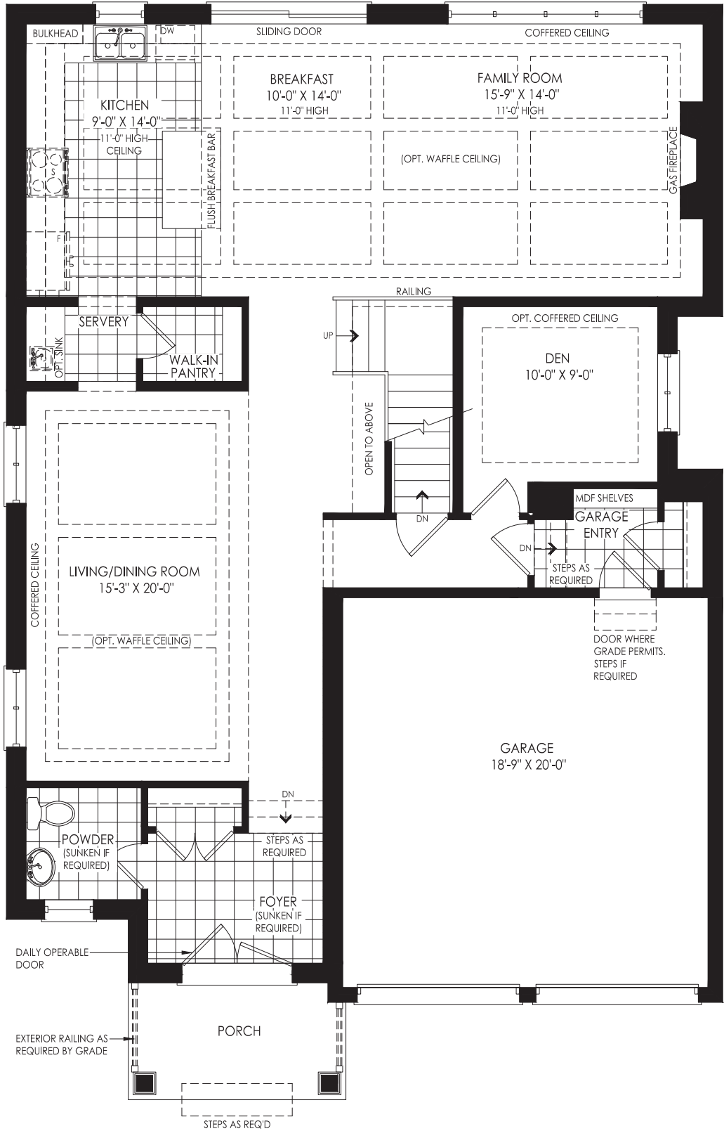
GROUND FLOOR PLAN ELEV. 'B'
