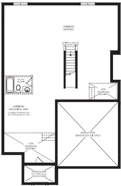
BASEMENT PLAN ELEV. 'B'
