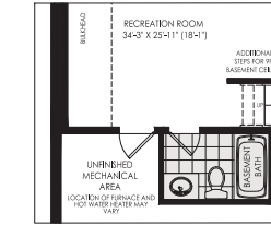
OPTIONAL FINISHED BASEMENT BATHROOM
