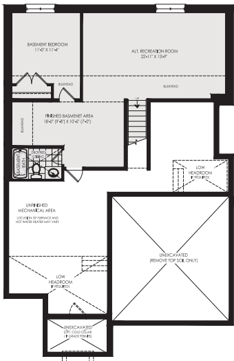
OPTIONAL FINISHED BASEMENT WITH RECREATION ROOM, BEDROOM AND BATHROOM ELEV. 'B'
