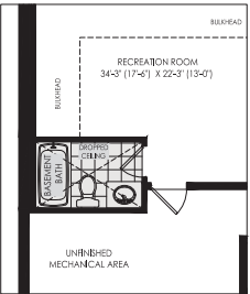
OPTIONAL FINISHED BASEMENT BATHROOM
