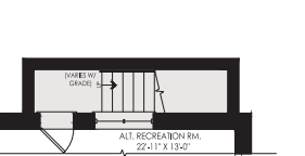
PARTIAL OPT. FINISHED BASEMENT PLAN W/ BASEMENT BEDROOM & BATHROOM FOR WALK- UP BASEMENT
