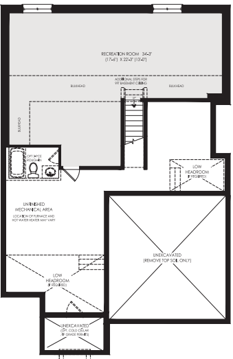
OPTIONAL FINISHED BASEMENT WITH RECREATION ROOM ELEV. 'B'
