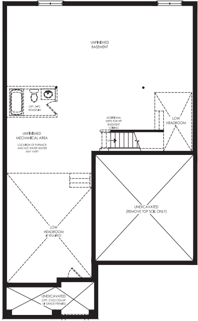
BASEMENT PLAN ELEV. 'C'
