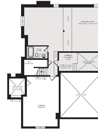
OPTIONAL FINISHED BASEMENT WITH RECREATION ROOM ELEV. 'A
