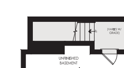
PARTIAL BASEMENT PLAN FOR WALK-UP BASEMENT
