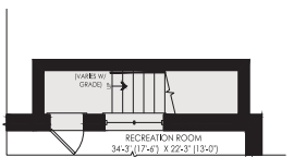
PARTIAL OPT. FINISHED BASEMENT PLAN FOR WALK-UP BASEMENT
