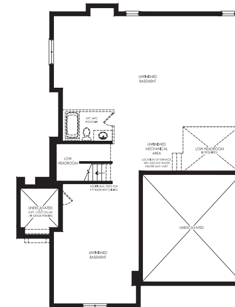
BASEMENT PLAN ELEV. 'A'
