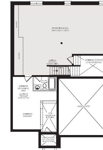
OPTIONAL FINISHED BASEMENT WITH RECREATION ROOM ELEV. 'A'
