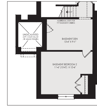
PARTIAL OPT. FINISHED BASEMENT PLAN W/ ALT. BASEMENT BEDROOM ELEV. 'A'
