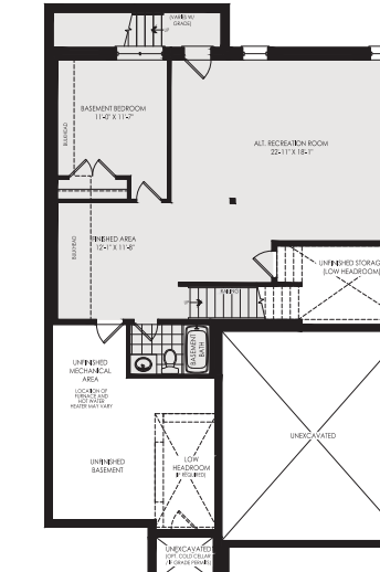
OPTIONAL FINISHED BASEMENT WITH RECREATION ROOM, BEDROOM AND BATHROOM & OPTIONAL WALK-UP BASEMENT STAIRS & OPTIONAL 9' BASEMENT CEILING HEIGHT ELEV. 'A'
