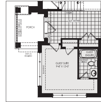
PARTIAL GROUND FLOOR OPT. GUEST SUITE ELEV. 'A'
