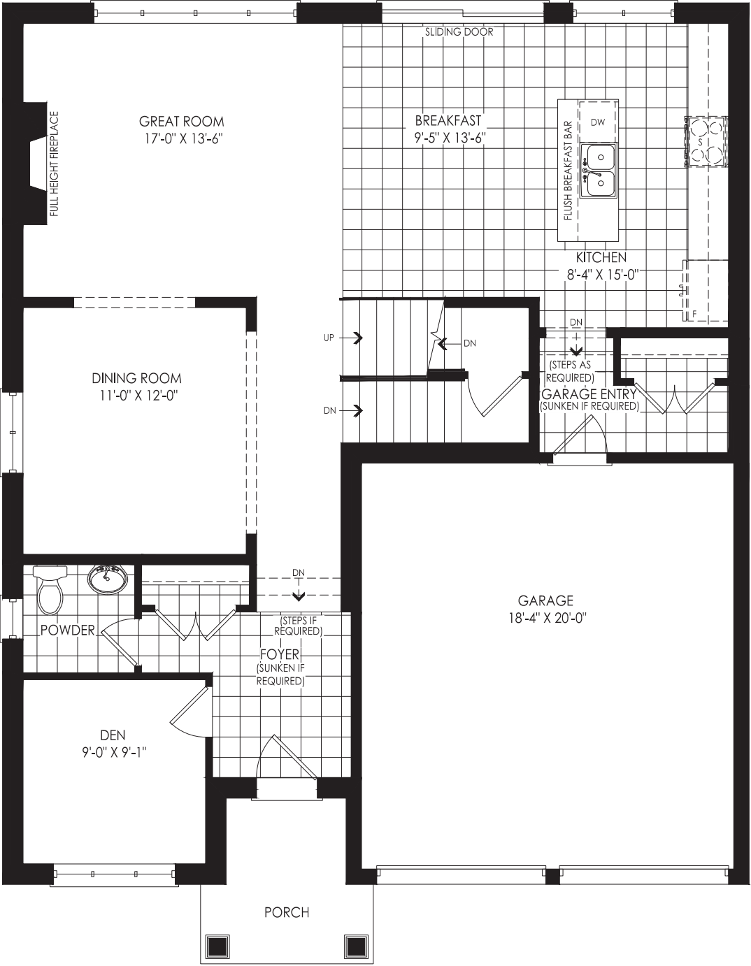
GROUND FLOOR PLAN ELEV. 'B'
