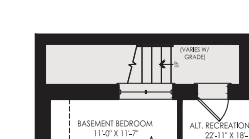
PARTIAL OPT. FINISHED BASEMENT PLAN W/ BASEMENT BEDROOM & BATHROOM FOR WALK- UP BASEMENT
