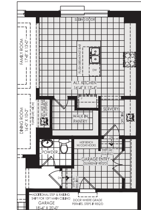
PARTIAL OPT. GROUND FLOOR W/ ALT. KITCHEN ELEV. 'A'
