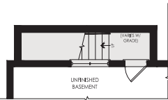
PARTIAL BASEMENT PLAN FOR WALK-UP BASEMENT
