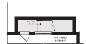
PARTIAL BASEMENT PLAN FOR WALK-UP BASEMENT
