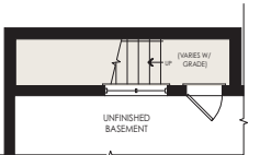
PARTIAL BASEMENT PLAN OPT. WALK-UP BASEMENT
