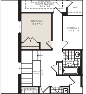
PARTIAL SECOND FLOOR PLAN OPT. 5 BEDROOM ELEV. 'A'
