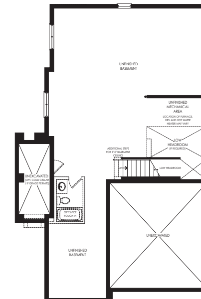
BASEMENT PLAN ELEV. 'A'
