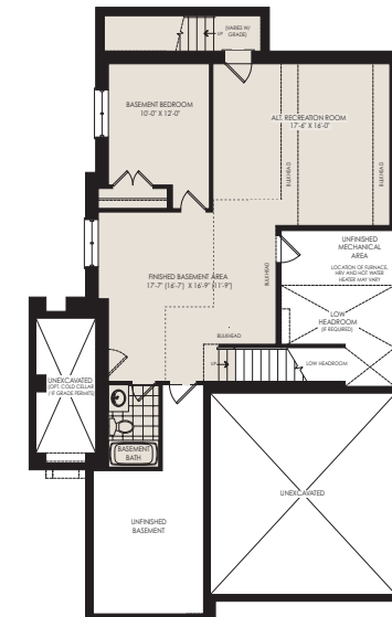
OPT. FIN. BASEMENT PLAN W/ BASEMENT BEDROOM, BATHROOM, WALK UP BASEMENT & 9FT BASEMENT CEILING HEIGHT ELEV. 'A'
