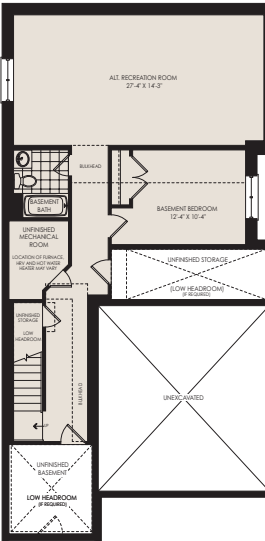
OPT. FINISHED BASEMENT PLAN W/ BASEMENT BEDROOM & BATHROOM ELEV. 'C' (STANDARD BASEMENT CEILING HEIGHT)
