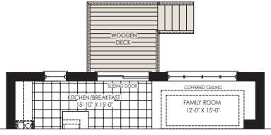
PARTIAL GROUND FLOOR ELEV. 'B' LOOKOUT BASEMENT CONDITION
