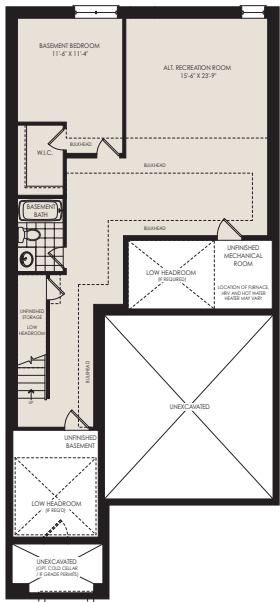
OPT. FINISHED BASEMENT PLAN W/ BASEMENT BEDROOM & BATHROOM, WALK UP (STANDARD BASEMENT CEILING HEIGHT)
