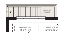
PARTIAL GROUND FLOOR FOR WALK-UP BASEMENT
