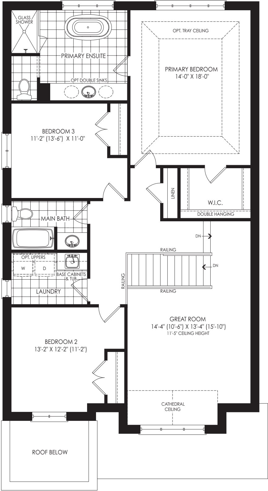
SECOND FLOOR PLAN ELEV. 'B'
