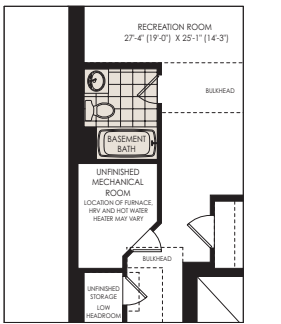
PARTIAL OPT. FINISHED BASEMENT PLAN W/ 3 P.C. BATHROOM ELEV. 'C'
