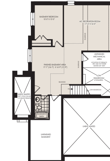
OPT. FINISHED BASEMENT PLAN W/ BASEMENT BEDROOM & BATHROOM ELEV. 'A' (STANDARD BASEMENT CEILING HEIGHT)
