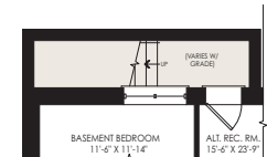
PARTIAL BASEMENT PLAN OPT. WALK-UP BASEMENT (FINISHED BASEMENT WITH BEDROOM & BATH CONDITION)
