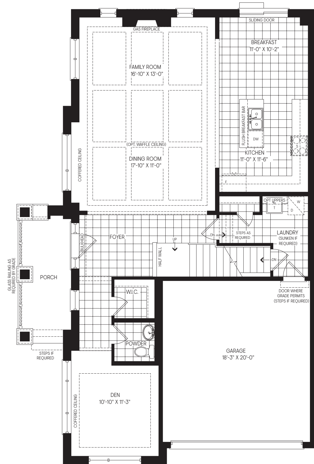
GROUND FLOOR PLAN ELEV. 'A'
