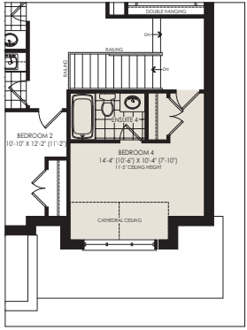
PARTIAL SECOND FLOOR PLAN OPT. 4 BEDROOM ELEV. 'B'
