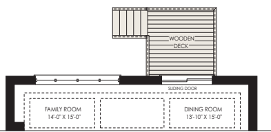
PARTIAL GROUND FLOOR ELEV. 'A' LOOKOUT BASEMENT CONDITION
