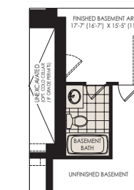
PARTIAL OPT. FINISHED BASEMENT PLAN W/ 3 PC. BATHROOM ELEV. 'A'
