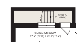
PARTIAL BASEMENT PLAN OPT. WALK-UP BASEMENT (FINISHED BASEMENT CONDITION)
