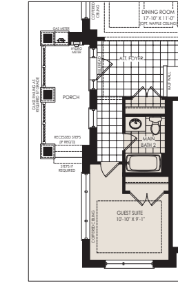
PARTIAL GROUND FLOOR PLAN OPT. GUEST SUITE ELEV. 'A'
