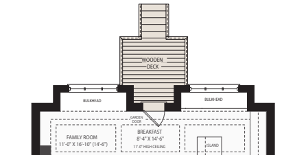
PARTIAL GROUND FLOOR ELEV. 'B' LOOKOUT BASEMENT CONDITION
