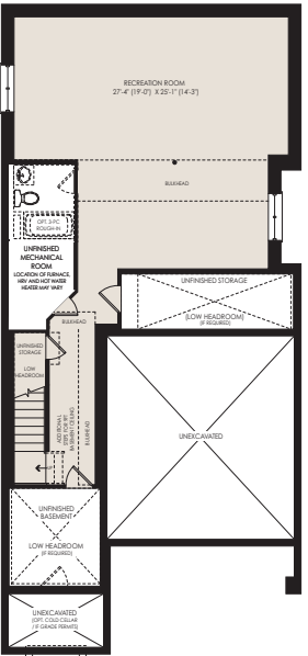
OPT. FINISHED BASEMENT PLAN ELEV. 'C'
