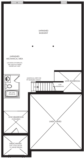
BASEMENT PLAN ELEV. 'B'
