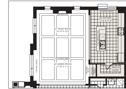
PARTIAL GROUND FLOOR PLAN OPT. ALT. KITCHEN ELEV. 'A'
