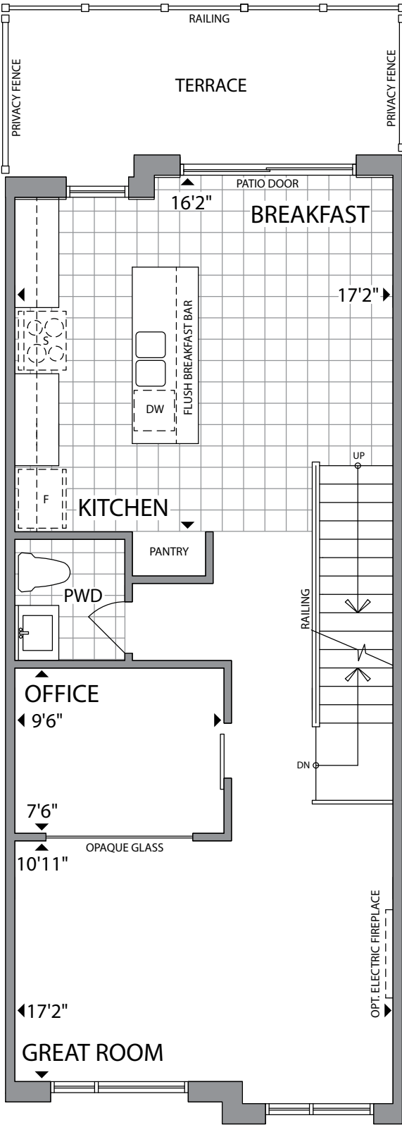
MAIN FLOOR ELEVATION A2
