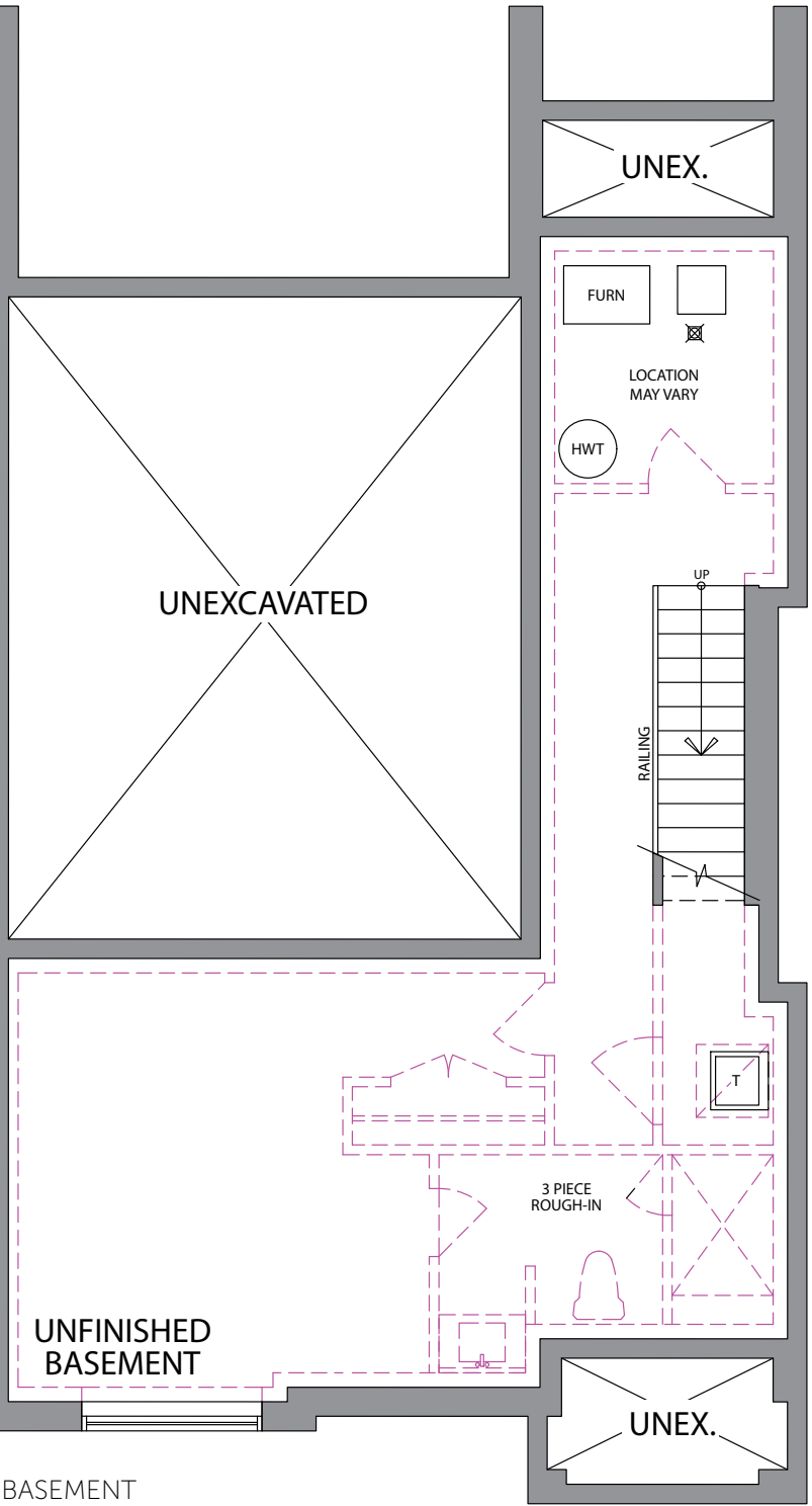
BASEMENT ELEVATION A1
