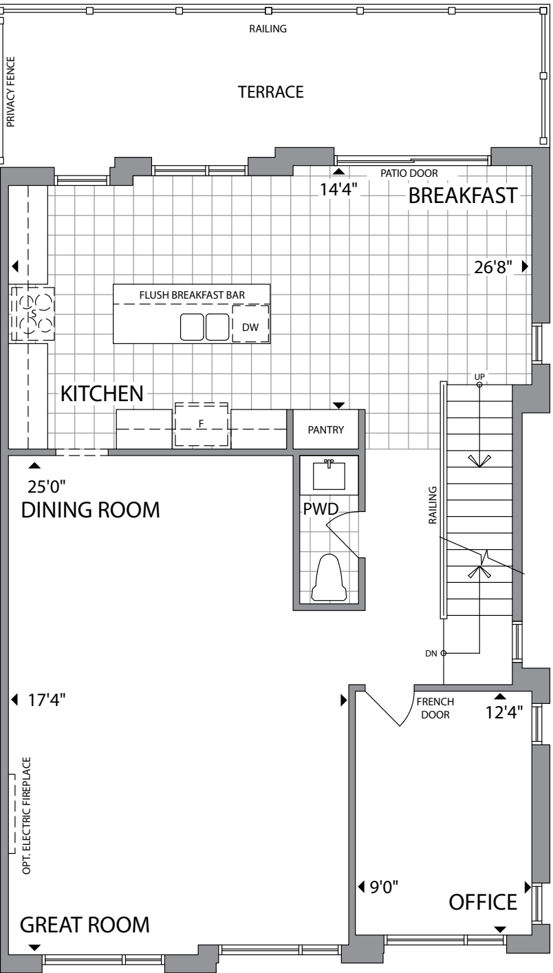
MAIN FLOOR ELEVATION A1
