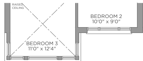
SECOND FLOOR ELEVATION C
