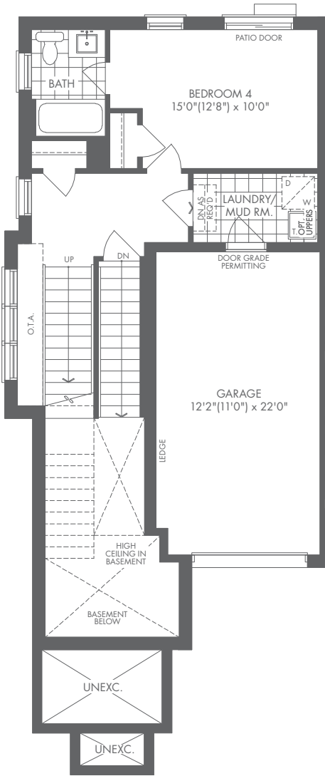
LOWER A
