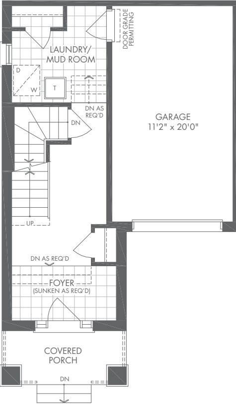
LOWER B
