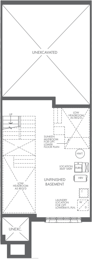
BASEMENT B
