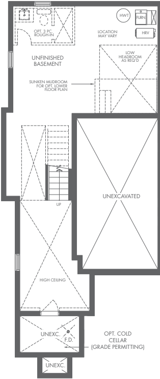
BASEMENT A
